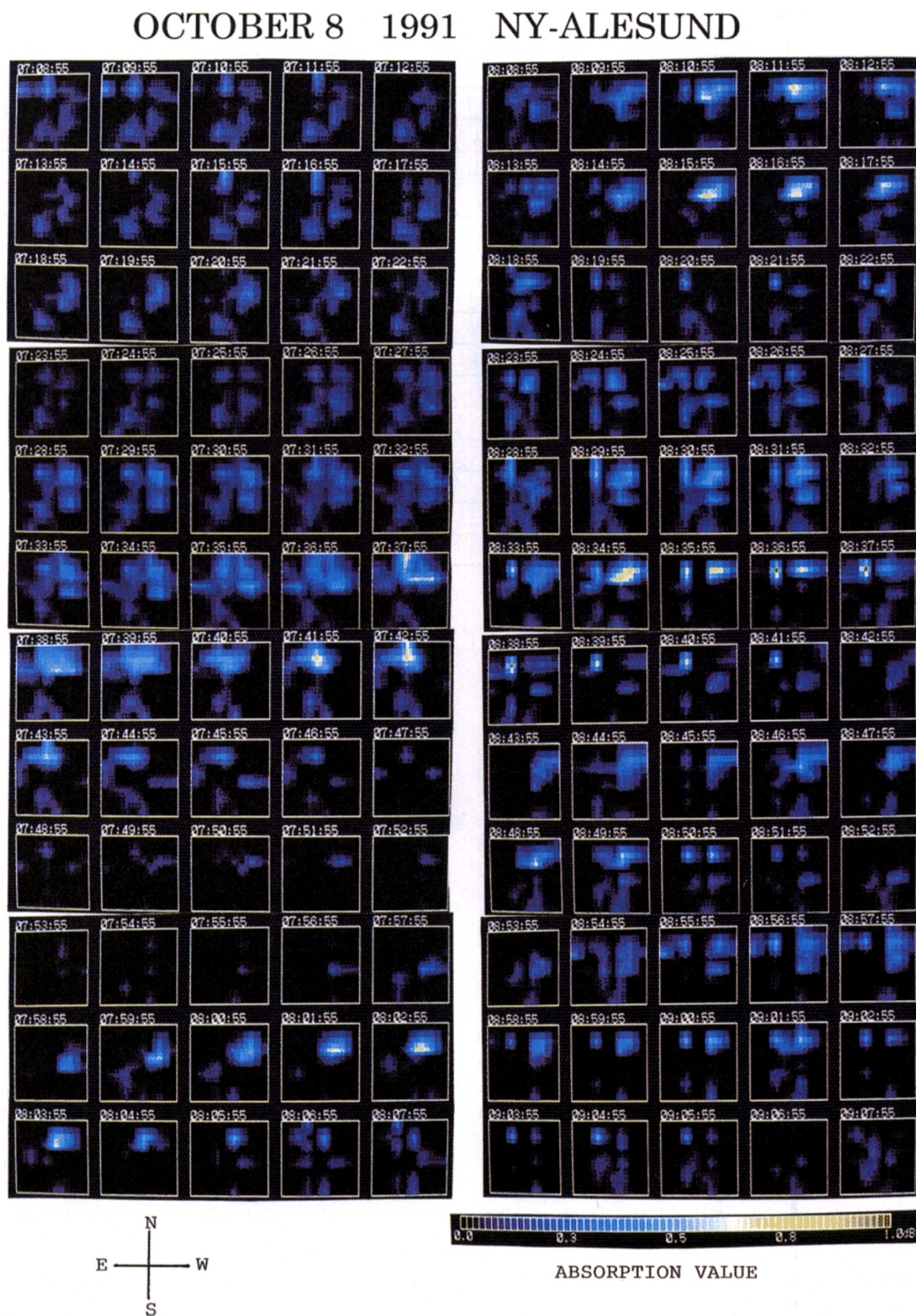
Plate 1. Time series of the absorption images, produced from the 64 IRIS beams, during 0708:56–0907:55 UT on October 8, 1991. Each image is an average over one minute. The absorption scale up to 1 dB is displayed by the color bar.
