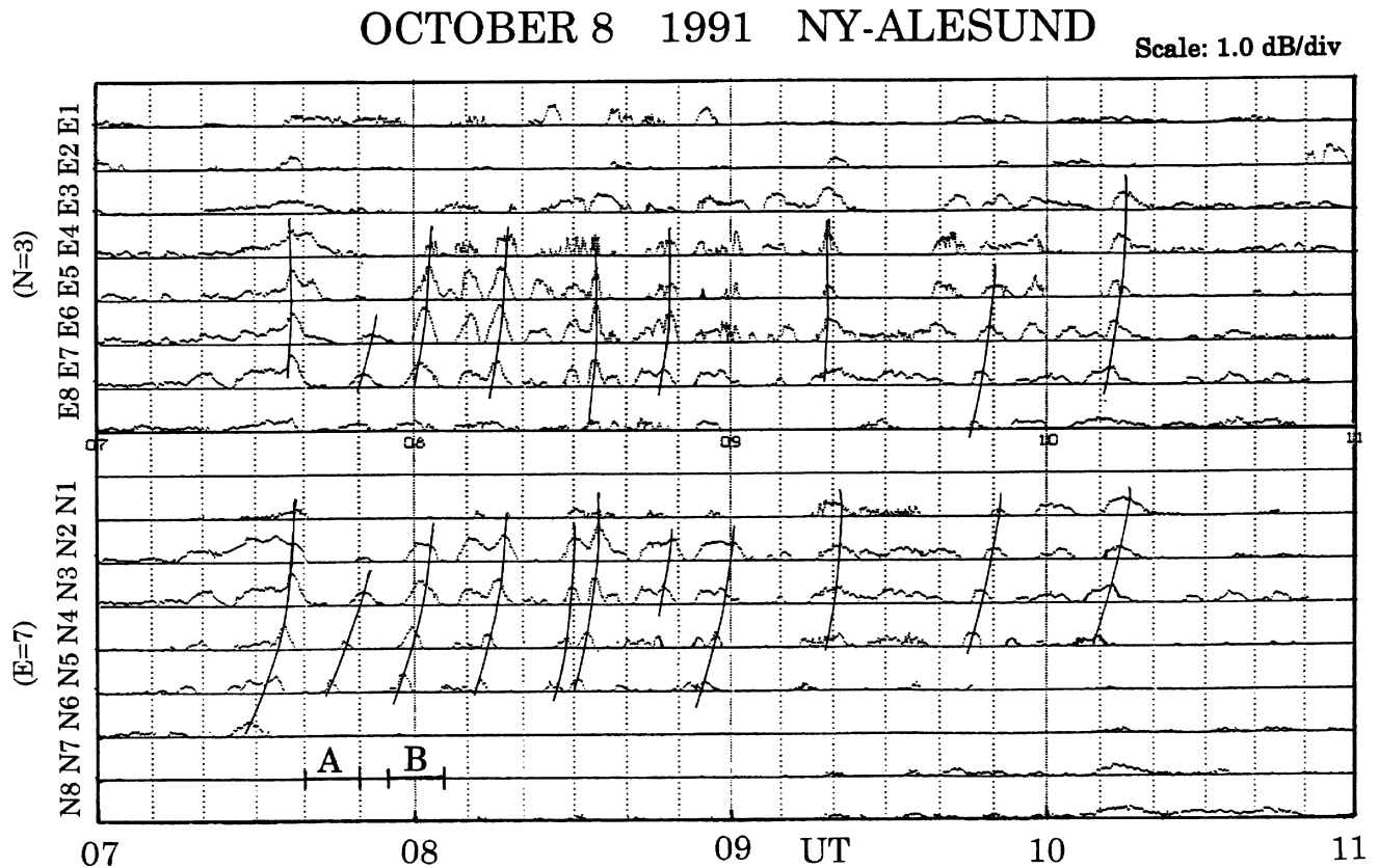
Fig. 2. The time-varying absorption intensities for the eight-beams in the east-west cross-section passing through the third-northernmost row (N3), and those in the north-south cross-section passing through the second-westernmost column (E7), observed at Ny-Alesund during 0700–1100 UT on October 8, 1991.
