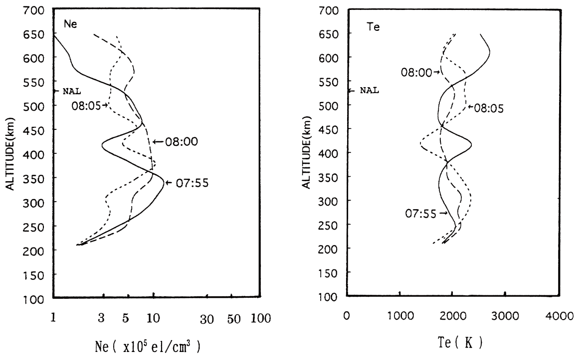
Fig. 6. Altitude profiles of electron densities (left panel) and electron temperatures (right panel) during 0755–0805 UT.
