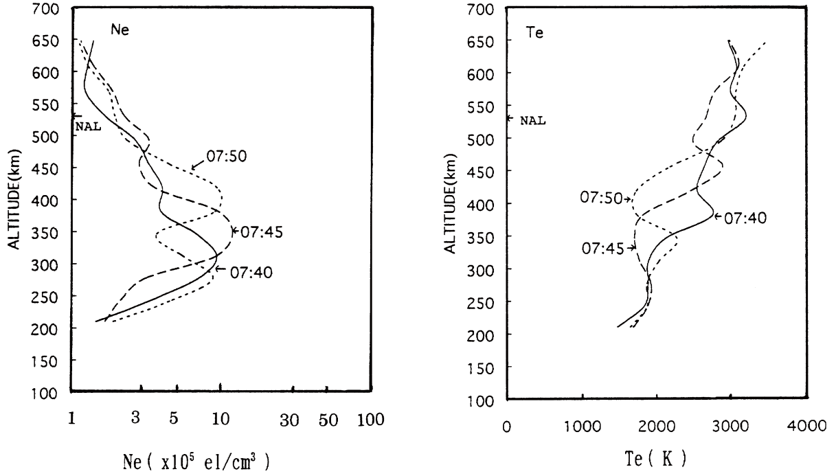
Fig. 5. Altitude profiles of electron densities (left panel) and electron temperatures (right panel) during 0740–0750 UT.
