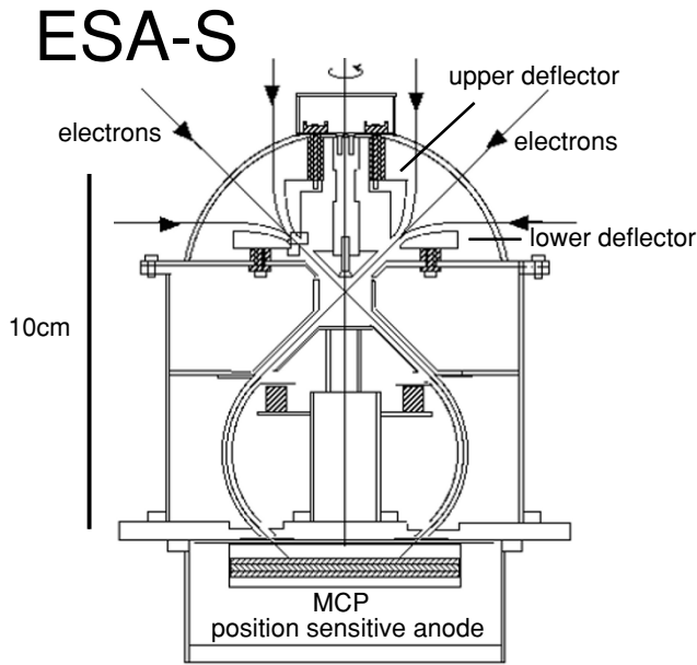
Fig. 1. Cross section of ESA-S1 and ESA-S2.
