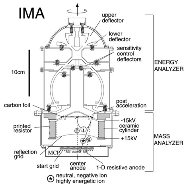
Fig. 2. Cross section of IMA.
