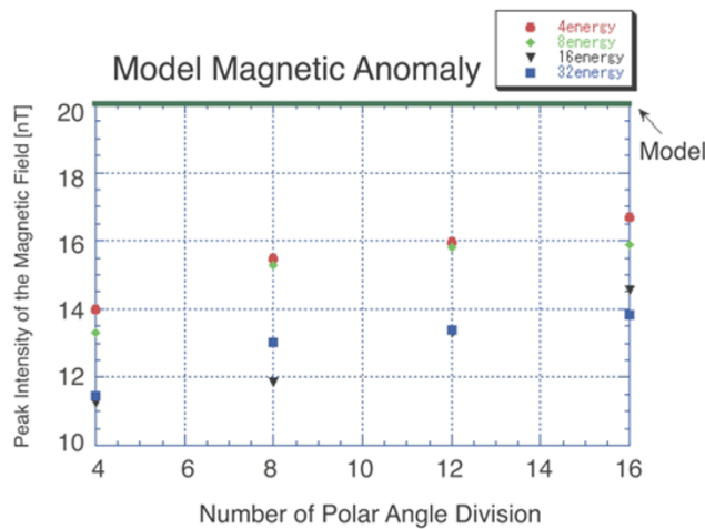
Fig. 10. Peak intensity of the measured magnetic anomaly with respect to the number of the polar angle division of 4, 8, 12 and 16. The estimated magnetic anomaly for the energy steps of 4, 8, 16, and 32 are shown.
