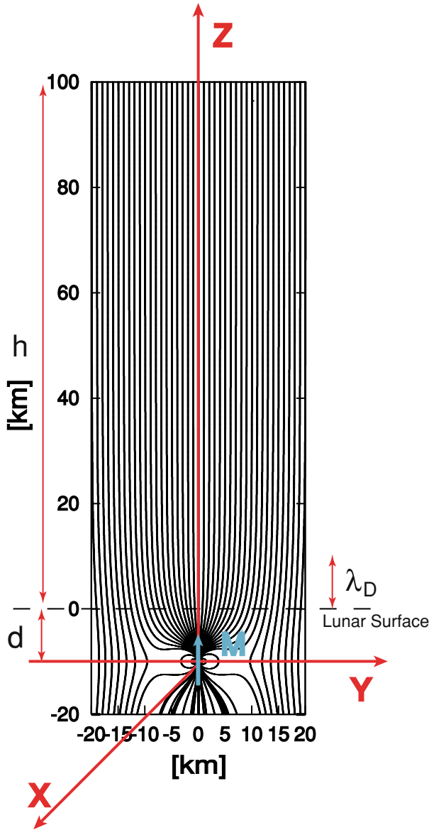
Fig. 6. Model magnetic anomaly on the lunar surface.
