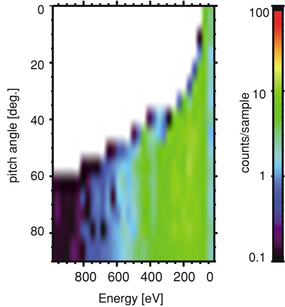
Fig. 7. Calculated pitch angle distribution of electrons.
