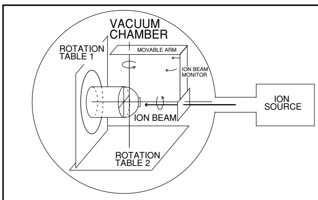
Fig. 4. A schematic diagram that shows the configuration of the calibration experiment.
