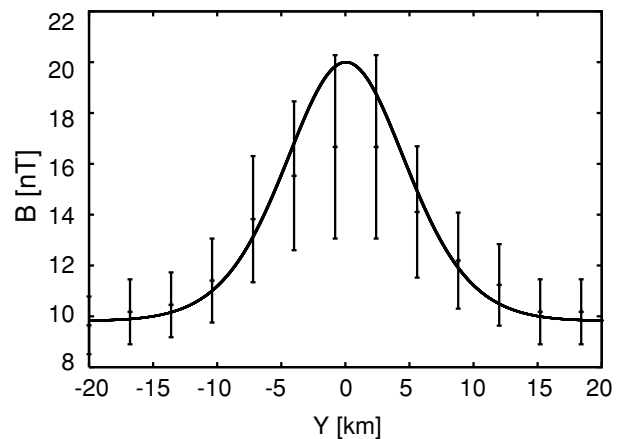
Fig. 8. Reproduced intensity of the magnetic anomaly when the number of measured energy steps was four and the number of polar angular division was 16.
