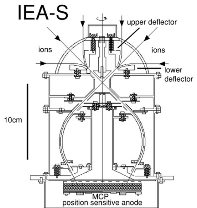
Fig. 3. Cross section of IEA.
