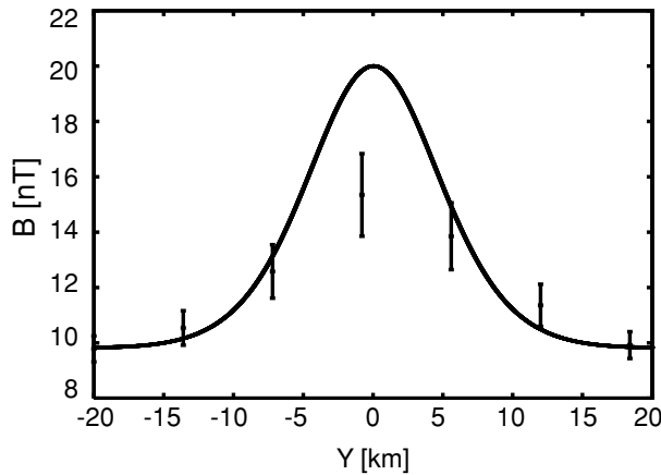
Fig. 9. Reproduced intensity of the magnetic anomaly when the number of measured energy steps was eight and the number of polar angular division was 16.
