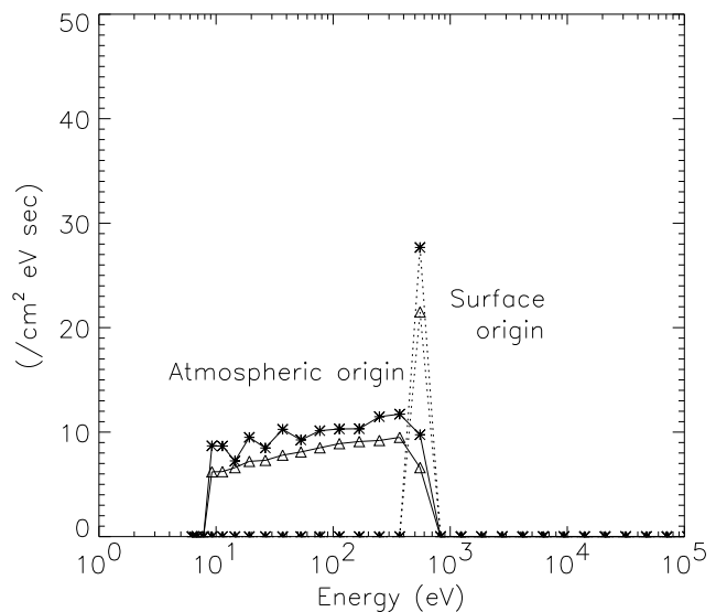
Fig. 5. Energy spectra of picked-up lunar \text{Na}^+ and \text{K}^+ ions at an altitude of 100 km. The asterisk and triangle denote \text{Na}^+ and \text{K}^+ , respectively. Solid and dashed lines denote ions of atmospheric origin and surface origin, respectively.
