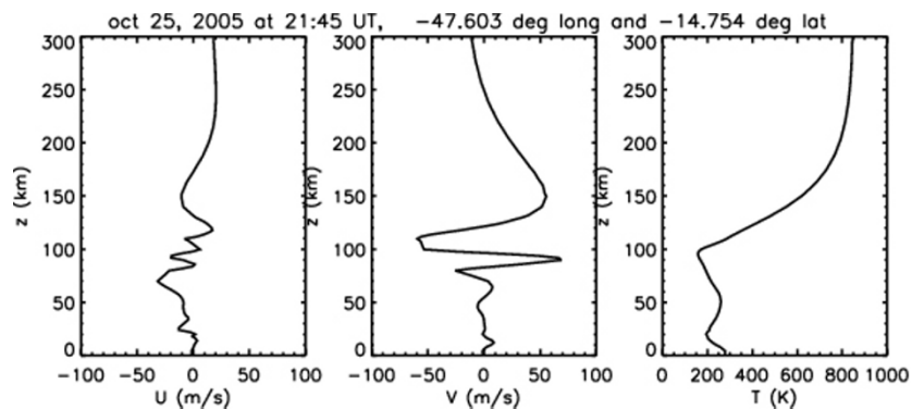
Fig. 4. Zonal (left) and meridional (center) wind and temperature (right) profiles at (47.6^\circ\text{W}, 14.75^\circ\text{S}) and 21:45 UT used for ray tracing GWs arising from the deep convective plumes observed in Fig. 3. The profiles were defined by balloon soundings below 30 km, meteor radar observations between 80 and 100 km, and a TIME GCM simulation initialized with the NCEP reanalysis data for this same period from 35 to 70 km and from 110 to 350 km, with linear interpolation elsewhere.
