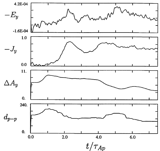
Fig. 9. The time histories of the toroidal electric field E_y and current J_y , the difference of the vector potential between the separatrix and flux bundles \Delta A_y , and the distance between the flux bundles d_{p-p} for the 3D reconnection.
