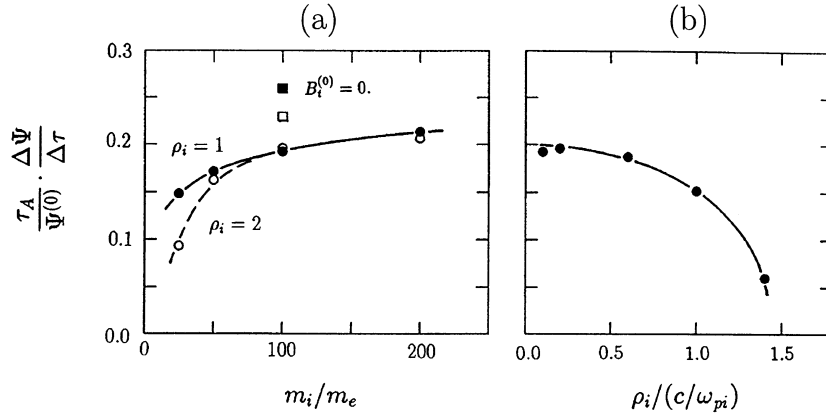
Fig. 7. The parametric dependences of the reconnection rate on (a) the ion mass (for \rho_i = 1, 2c/\omega_{pe} ), and (b) the ion Larmor radius (for m_i/m_e = 100 ). Also in (a), the reconnection rates for the applied toroidal magnetic field of B_t = 0 and 0.2 are plotted with solid and open squares, respectively.
