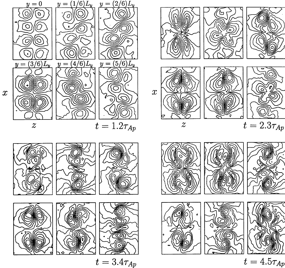
Fig. 11. Snapshots of the scalar potential \varphi ( \mathbf{E}_p = -\nabla\varphi ) at six cross sections along the y -direction (the order is from left to right, then top to bottom), at four times t/\tau_A = 1.2, 2.3, 3.4 and 4.5 .
