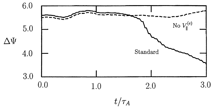
Fig. 5. Time history of the isolated poloidal flux for the standard run (solid), and for the special run (dashed) in which spatial displacement of electrons along the magnetic field is discarded while keeping the toroidal current, i.e. the MHD case.
