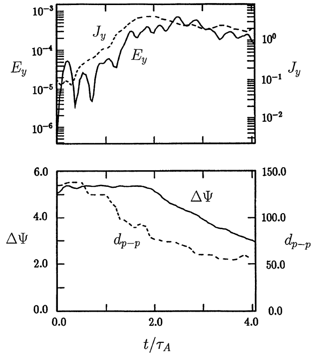
Fig. 3. Time histories of the toroidal electric field E_y , and the toroidal current J_y in the upper panel, and those of the isolated poloidal flux \Delta\Psi contained in the flux bundles, and the distance between the flux bundle centers d_{p-p} in the lower panel. These quantities except d_{p-p} are measured at the separatrix, and the signs of E_y and J_y are reversed.
