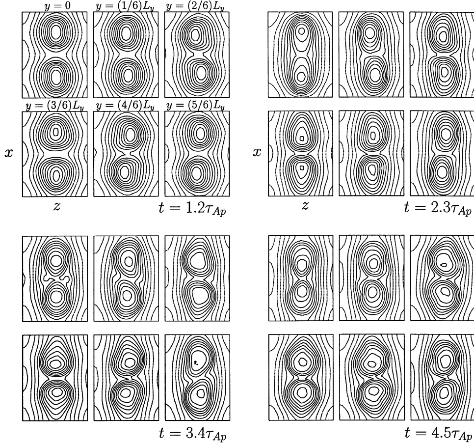
Fig. 10. Snapshots of the y -component of the vector potential A_y at six cross sections along the y -direction (the order is from left to right, then top to bottom), at four times t/\tau_A = 1.2, 2.3, 3.4 and 4.5 .
