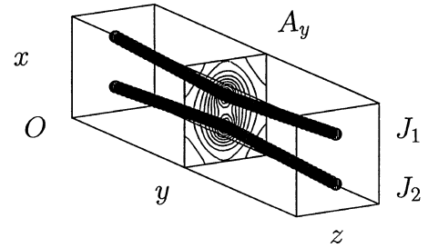
Fig. 8. Schematic illustration of the geometry for the 3D simulation. The dots represent the axial current J_1 and J_2 carried by ions, and contours on the poloidal cross section show the y -component of the vector potential A_y .
