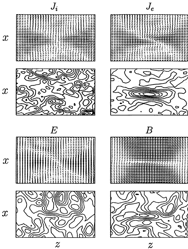
Fig. 12. Enlarged plots of the poloidal quantities in the vicinity of the separatrix at t = 2.3\tau_A of Fig. 9 (plot format is the same as that of Fig. 4). The ion and electron currents J_i and J_e in the top row, and the electric and magnetic fields E , B in the bottom row. In each group, the upper and lower panels correspond to the poloidal and toroidal components, respectively.
