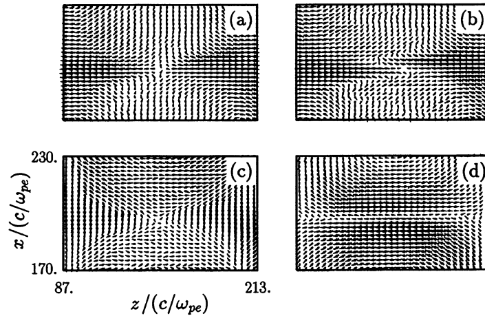
Fig. 4. Enlarged plots of the poloidal quantities in the vicinity of the separatrix (in a small rectangular box of Fig. 2(b)). The ion and electron currents in (a) and (b), respectively, and the electric and magnetic fields in (c) and (d).
