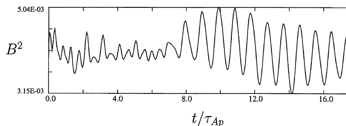
Fig. 13. Oscillations in the magnetic energy B^2 on a long time scale, which are mainly due to the toroidal component of the magnetic field.
