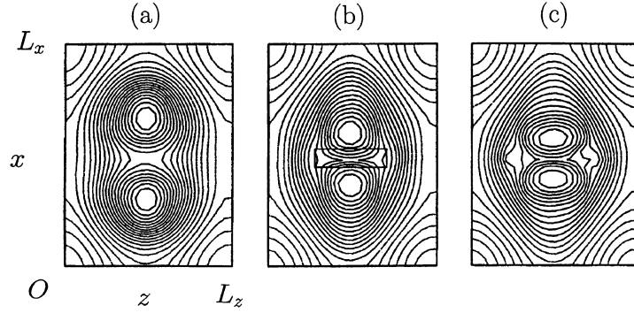
Fig. 2. Snapshots of the poloidal flux function in (a) the equilibrium state t = 0.75\tau_A , (b) the most active phase of reconnection t = 1.9\tau_A and (c) t = 2.5\tau_A .
