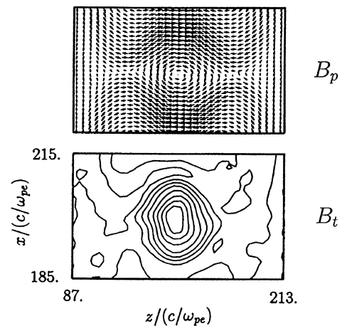
Fig. 6. The poloidal and toroidal magnetic field for the special run in Fig. 5 at t = 3\tau_A . The plasmoid stays at the separatrix and impedes magnetic reconnection.
