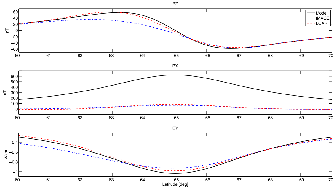
Fig. 3. Profiles of the surface electric and magnetic fields along longitude 23^{\circ} East (see Fig. 2) for a simple 1D electrojet model. Top panel shows the vertical magnetic field, middle panel the horizontal (North component) magnetic field and bottom panel the horizontal (East component) electric field. The model distribution is plotted with solid line, and the results calculated using IMAGE and BEAR stations (see Fig. 2) with dash-dotted and dashed lines, respectively.
