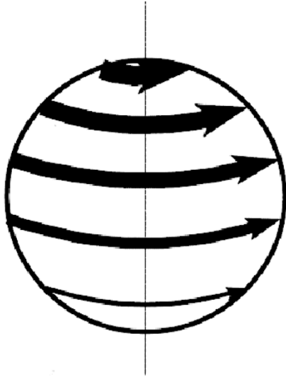
Fig. 1. Divergence-free Spherical Elementary Current System (SECS). From Amm and Viljanen (1999).
