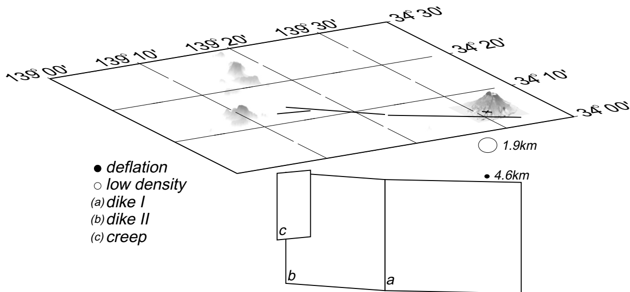
Fig. 5. 3-D view of source model for the ground displacements and gravity changes which are caused by the 2000 Miyakejima volcanic unrest and ground displacements nearby Izu-islands, Japan. Five elements are used, i.e., (i) Mogi-type deflation source, (ii) Lightened body, (iii) Tensile dislocation I, (iv) Tensile dislocation II and (v) Strike slip fault. The depth of the top edge of tensile dislocation I is 1000 m, and its height is 10 km; see Table 1 for details. The elevation map of the Izu-islands is based on GSI's digital elevation models of 50-meter resolution except at Miyakejima, whose resolution is 10-meter.
