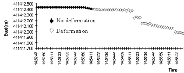
Fig. 1(b). Deformation detected with 3 second observations in E.
