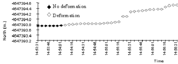
Fig. 2(a). Deformation detected with 5 second observations in N.
