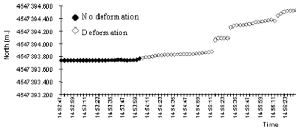
Fig. 2(b). Deformation detected with 3 second observations in N.
