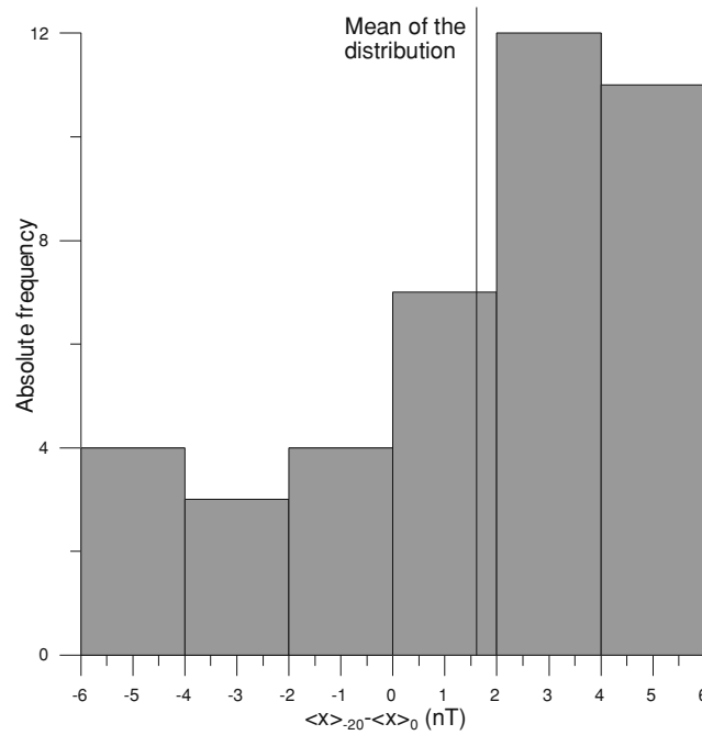
Fig. 5. Histogram showing the distribution of the 41 possible differences of the means after extraction of 20-minute-long gaps from the hourly interval 18:00–19:00 UT, January 9th, 2004, station LIV.
