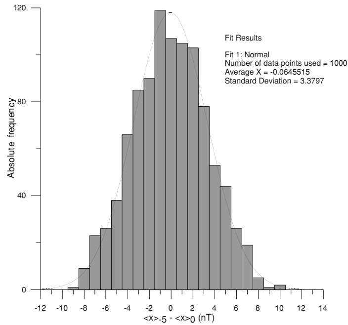
Fig. 2. Histogram showing the distribution of the 1000 differences of the means obtained after random extraction of 5 data points for a high-latitude observatory (CMO) and high activity level (A); hourly interval: January 17th, 2005, 09:00–10:00 UT.
