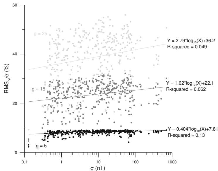
Fig. 7. Relative standard uncertainty, \text{RMS}_{-g}/\sigma , as a function of \sigma for the 360 hourly intervals after extraction of gap segments of length g = 5, 15 and 25 .
