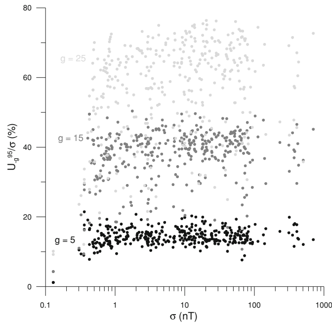
Fig. 8. Equivalent to Fig. 7 for the 95th percentile case.
