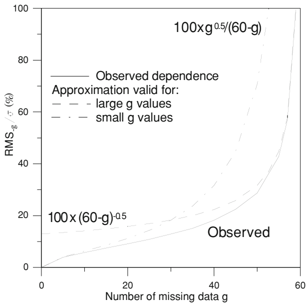
Fig. 4. Observed relative standard deviation after random extraction of g data points, together with approximations for large and small g values.
