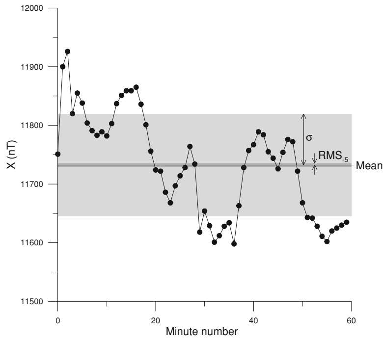
Fig. 1. X -component minute values of the disturbed hourly interval recorded at the CMO observatory on January 17th, 2005, 09:00–10:00 UT. The standard deviation \sigma and the RMS value obtained after random extraction of 5 data points are also displayed.
