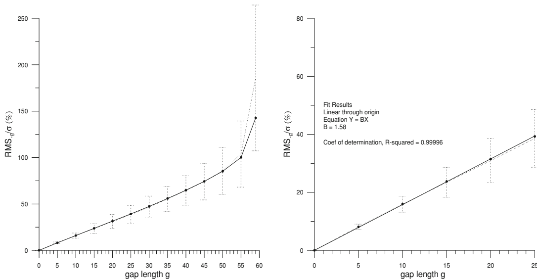
Fig. 10. The left-hand graph shows the standard uncertainty of the relative differences after extraction of different gap lengths g , whereas the right-hand plot shows a zoom for small and moderate g values. Discontinuous lines show the distribution of the relative standard uncertainties and error bars on them bound the central 68% of analyzed hours (results from the ‘individual’ analysis); solid lines correspond to the standard uncertainty determination of the overall distribution of the relative differences (results from the ‘simultaneous’ analysis).
