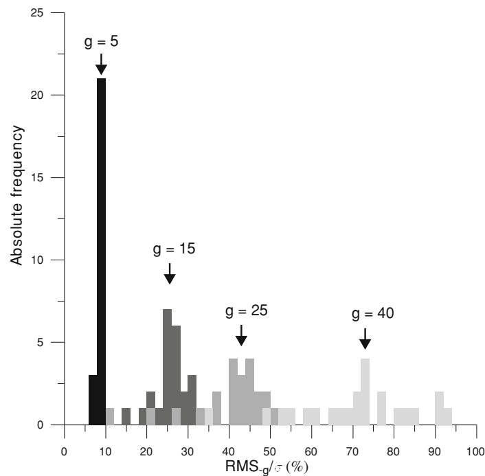
Fig. 6. Distribution of the individual RMS_{-g}/\sigma values ( g = 5, 15, 25 and 40 ) for the 24 hourly intervals of LIV M (moderate magnetic activity). For a gap length g = 15 , for example, most of the 24 estimated means are between 20 and 30% of \sigma away from the actual mean.
