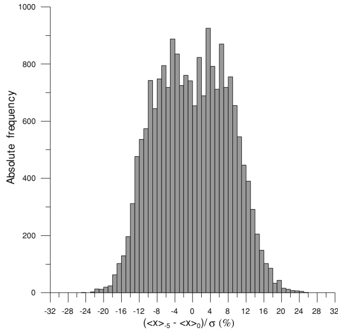
Fig. 9. Distribution of the 20160 relative differences obtained as a result of a simultaneous analysis for the whole set of hourly intervals for a gap length g = 5 .
