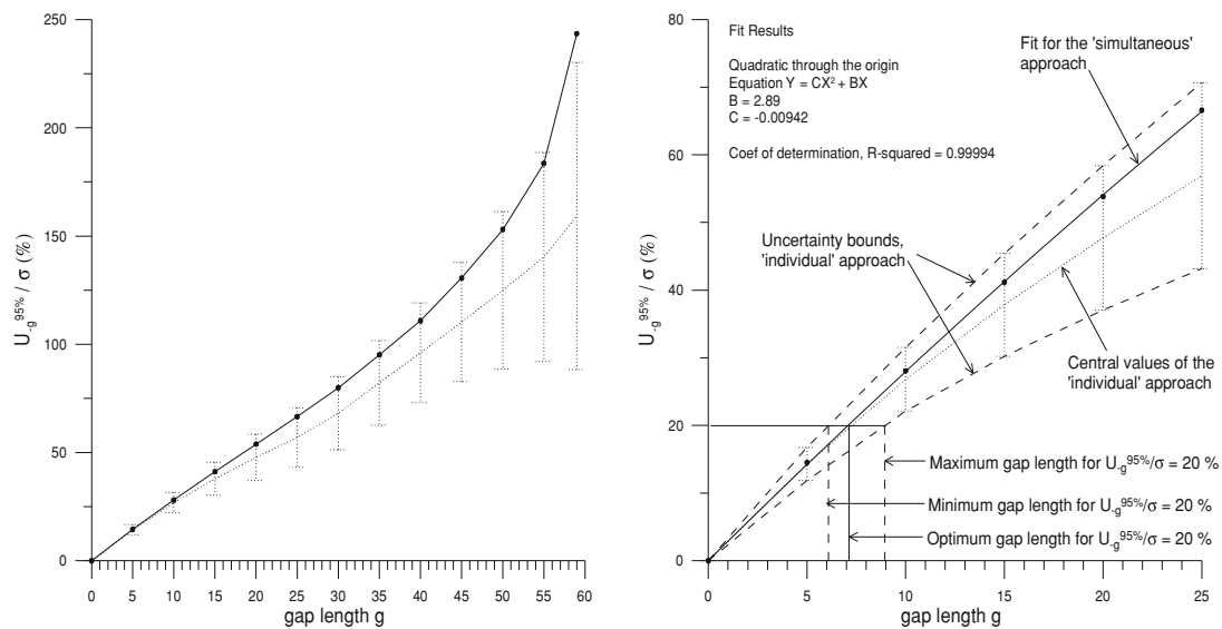
Fig. 11. Same as Fig. 10 for the relative 95% confidence level. Uncertainty bounds have been placed around the ‘individual’ approach central values, so as to include the 68% of the analyzed hourly intervals (i.e., 245). As an example, the correspondence between a particular value of U_{-g}^{95} (20% of \sigma ) and its associated gap length (between 6 and 9, with a maximum probability corresponding to 7) is outlined.
