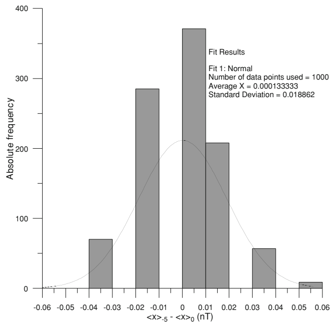
Fig. 3. Distribution of the 1000 means after random extraction of 5 data points for the hourly interval 00:00–01:00, Nov 16th, 2005, for SJG Q (quiet). Note that the Gaussian curve does not fit the observed data well. The striped structure of the distribution is an effect of the limited resolution of the primary minute data applied to such an extremely quiet interval.
