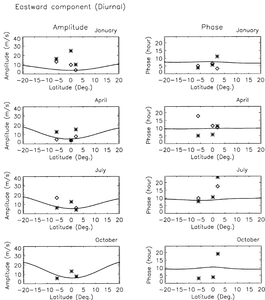
Fig. 6. Latitudinal sections of amplitudes (left) and phases (right) of diurnal tides at 90 km for (a) the eastward and (b) the northward wind velocity at Jakarta ( 6^{\circ}\text{S} ), Pontianak ( 0^{\circ} ) and Christmas Island ( 2^{\circ}\text{N} ). Four panels (from top to bottom) correspond to the determinations in January, April, July and October, and asterisks and squares indicate observations in 1996 and 1997, respectively.
